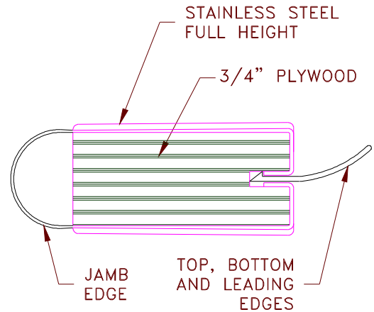
SECTION "AA" OF DOOR
