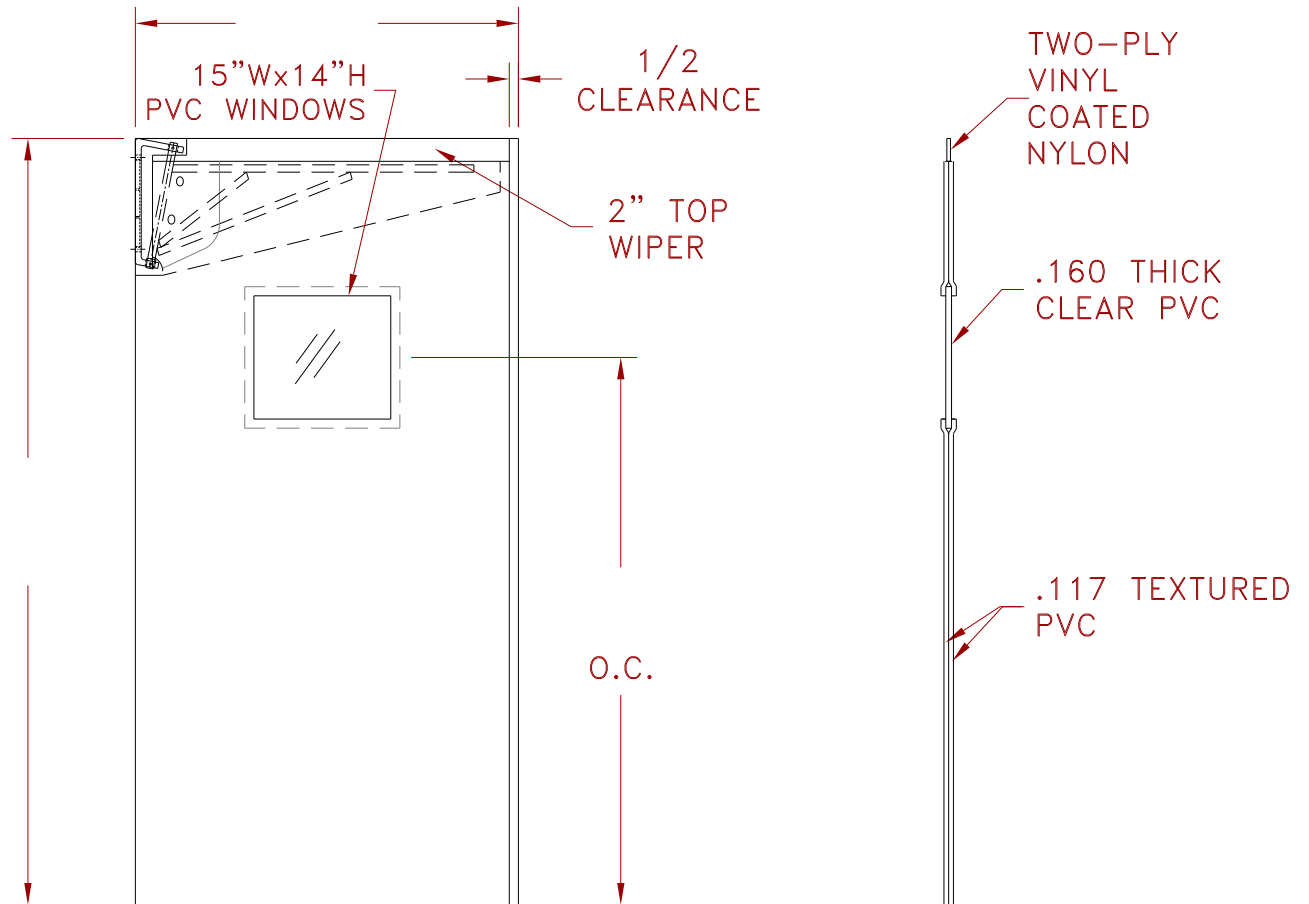
SIDE VIEW - 240
