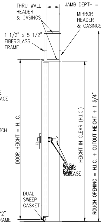
SIDE VIEW SECTION
