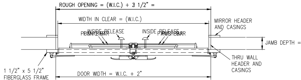
HORIZONTAL SECTION
