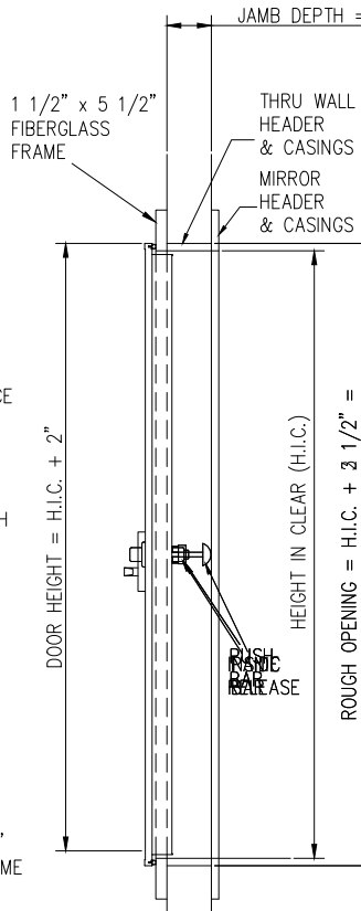
SIDE VIEW SECTION
