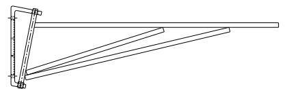
TOP MOUNTED GRAVITY HINGE
