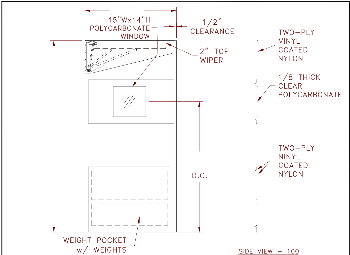
SIDE VIEW - 100
