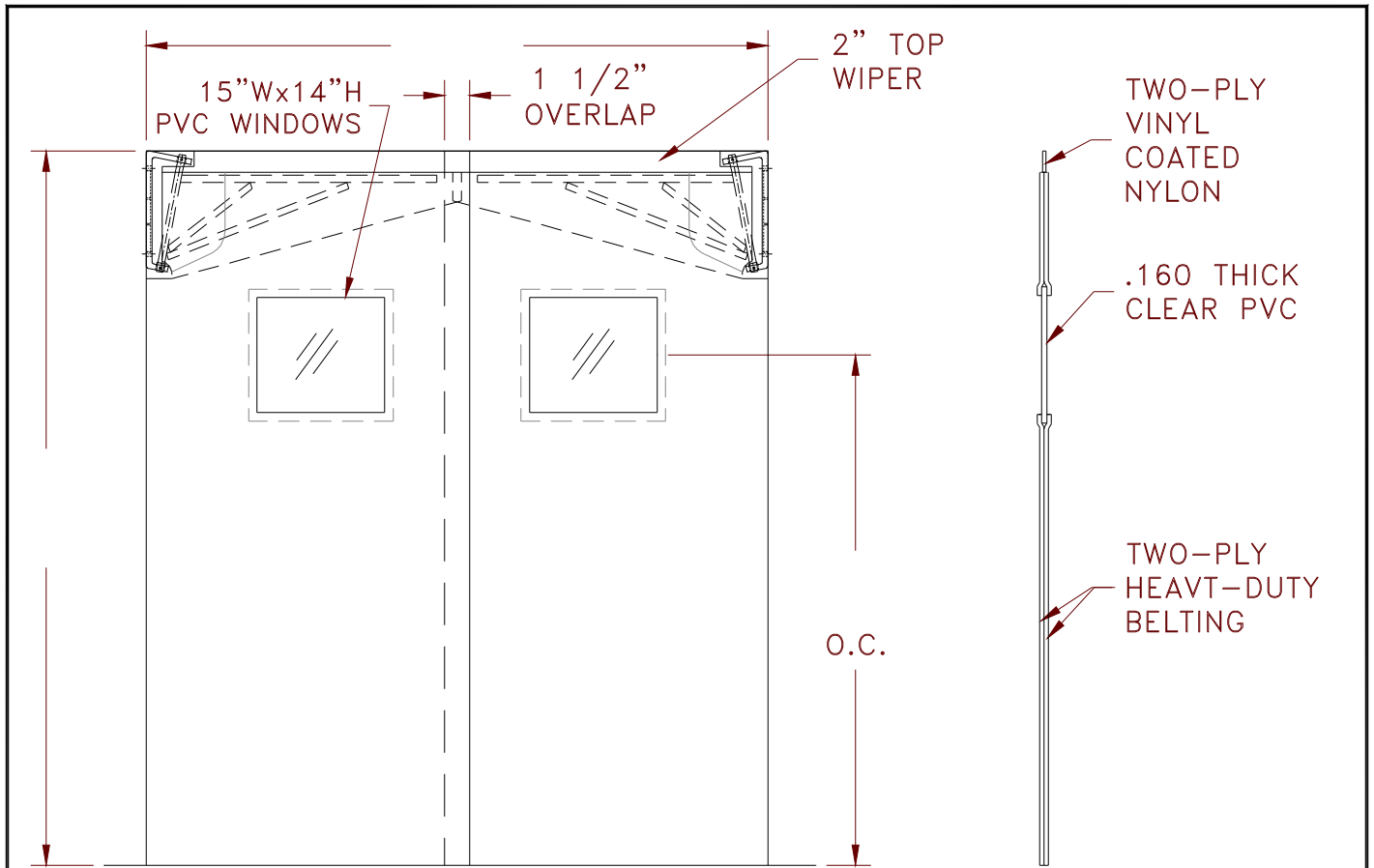
SIDE VIEW - 300
