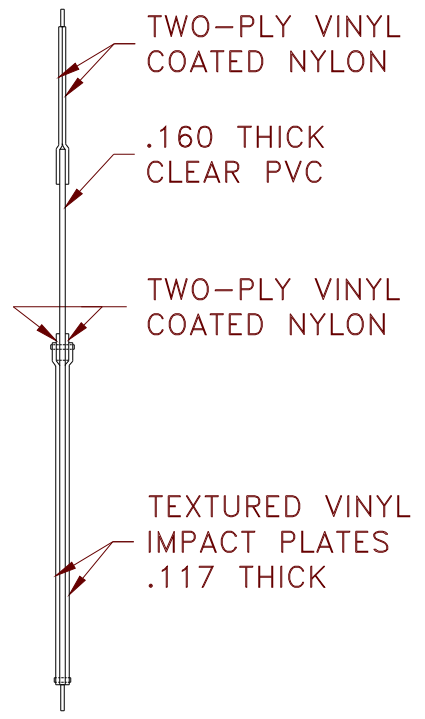
SIDE VIEW - 973
