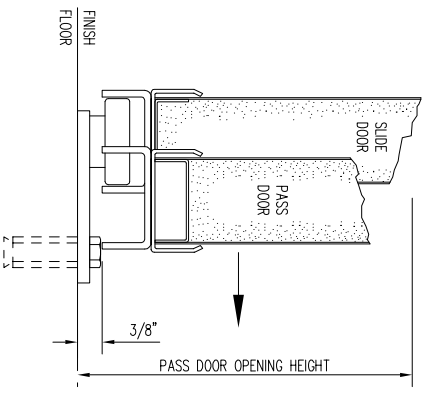
A PASS DOOR FRAME SECTION
