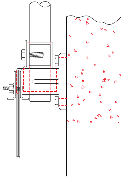
SECTION "A"
