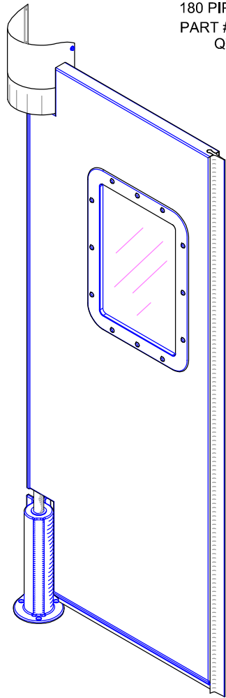
D05GS01628 1628 (STD Leading Edge Single)
