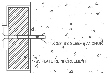
EXISTING MASONRY ANCHOR
