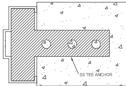
NEW MASONRY TEE ANCHOR
