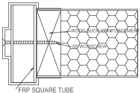
FRP SQUARE TUBE INSULATED PANEL WALL ANCHOR
