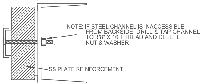
SS MACHINE SCREW ANCHOR
