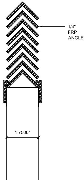
FRP LOUVER DETAIL
