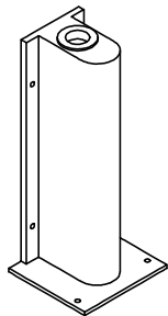
LOWER HINGE GUARD "Aluminum" PART # D05ASHGRCT QTY: _____
