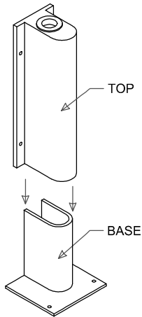
ADJUSTABLE HINGE GUARD "Aluminum ONLY" PART # D05KTADJLH QTY: _____
