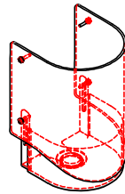
"NEW STYLE" UPPER HINGE SEAL PART # D05KTHS008 (KIT) PART # D05PPHSRAP (SEAL) QTY: _____
