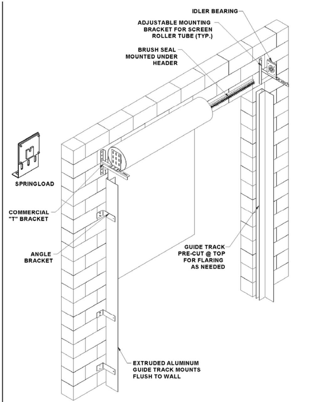
SPRINGLOAD FACE OF WALL GENERAL MOUNTING DIAGRAM
